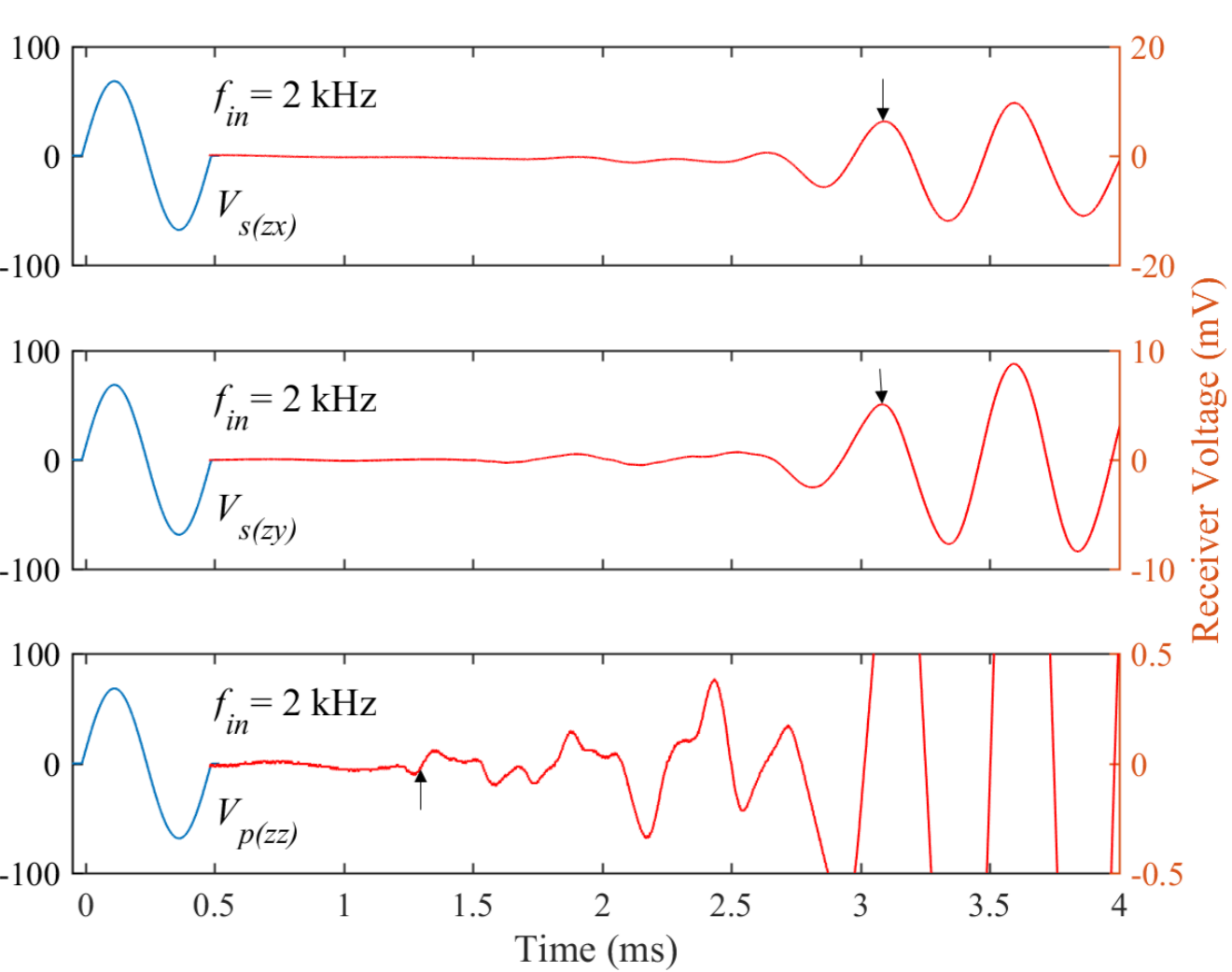
Time domain responses ( p' = 50 kPa)
