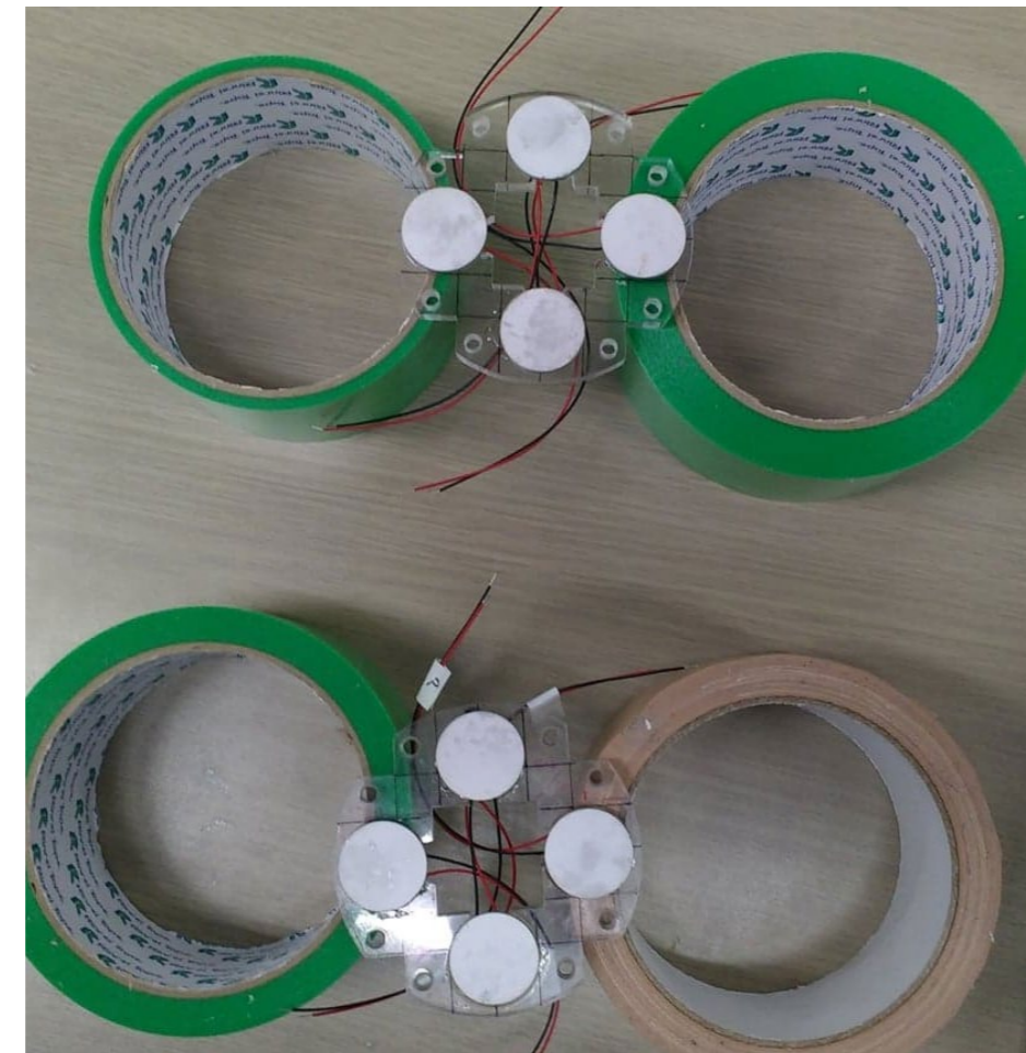
P-plate glued to acrylic disk
