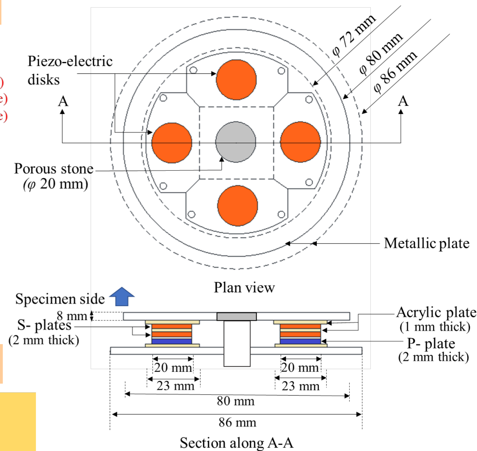
Schematic of vertical DT
