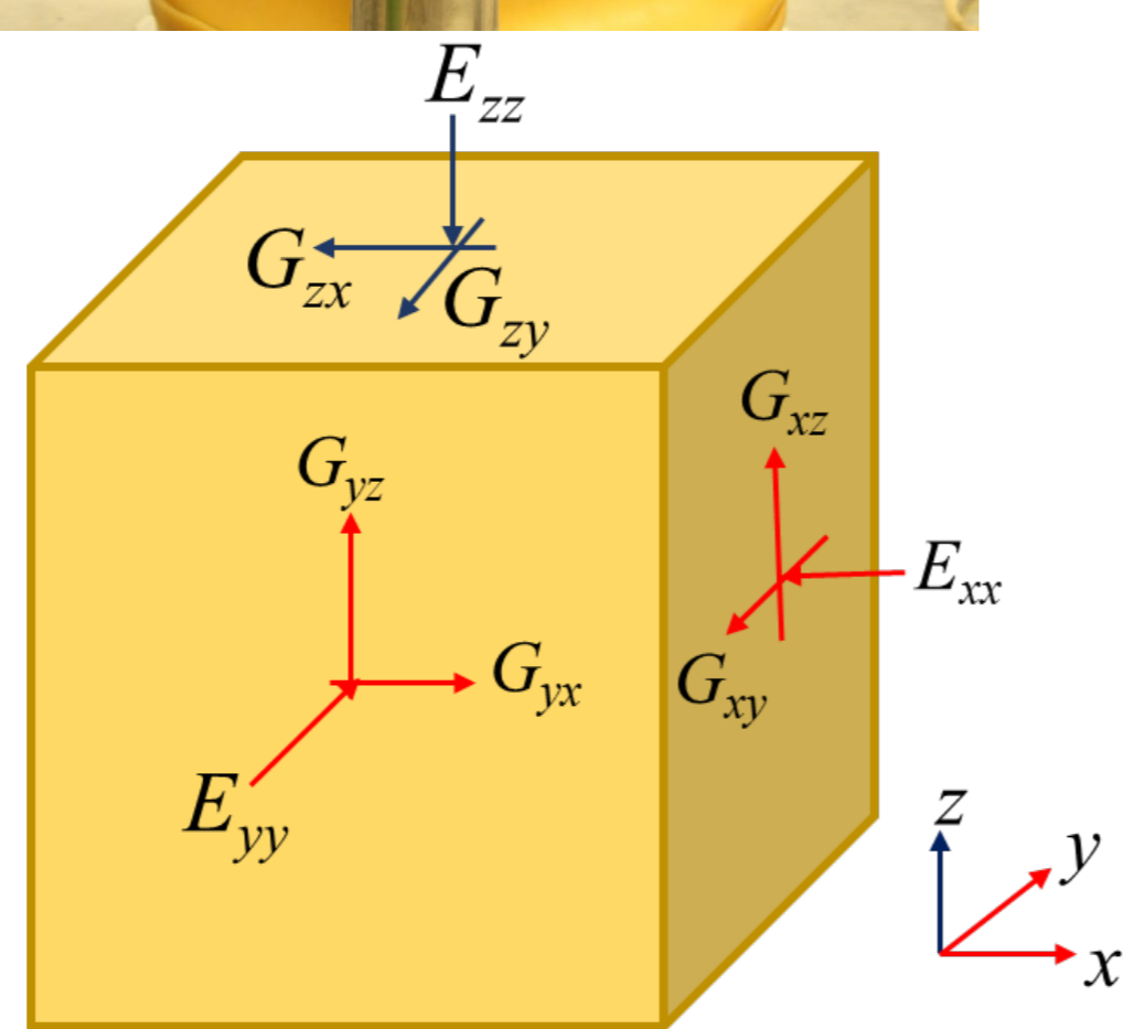
Notation of multidirectional stiffness
