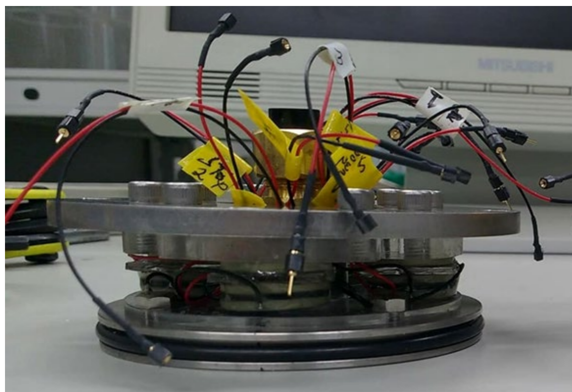
Transmitter assembly
