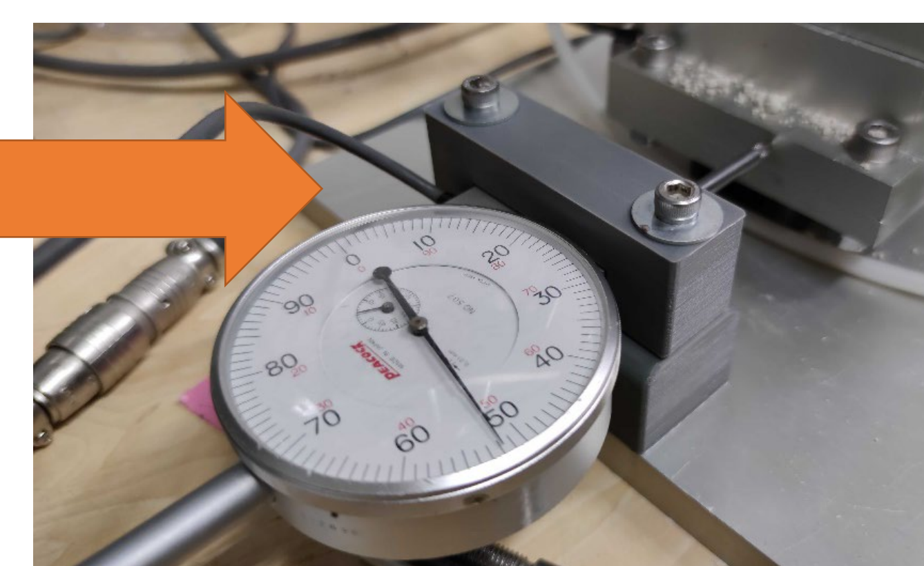
For Displacement Gauge, To Hold and Protect
