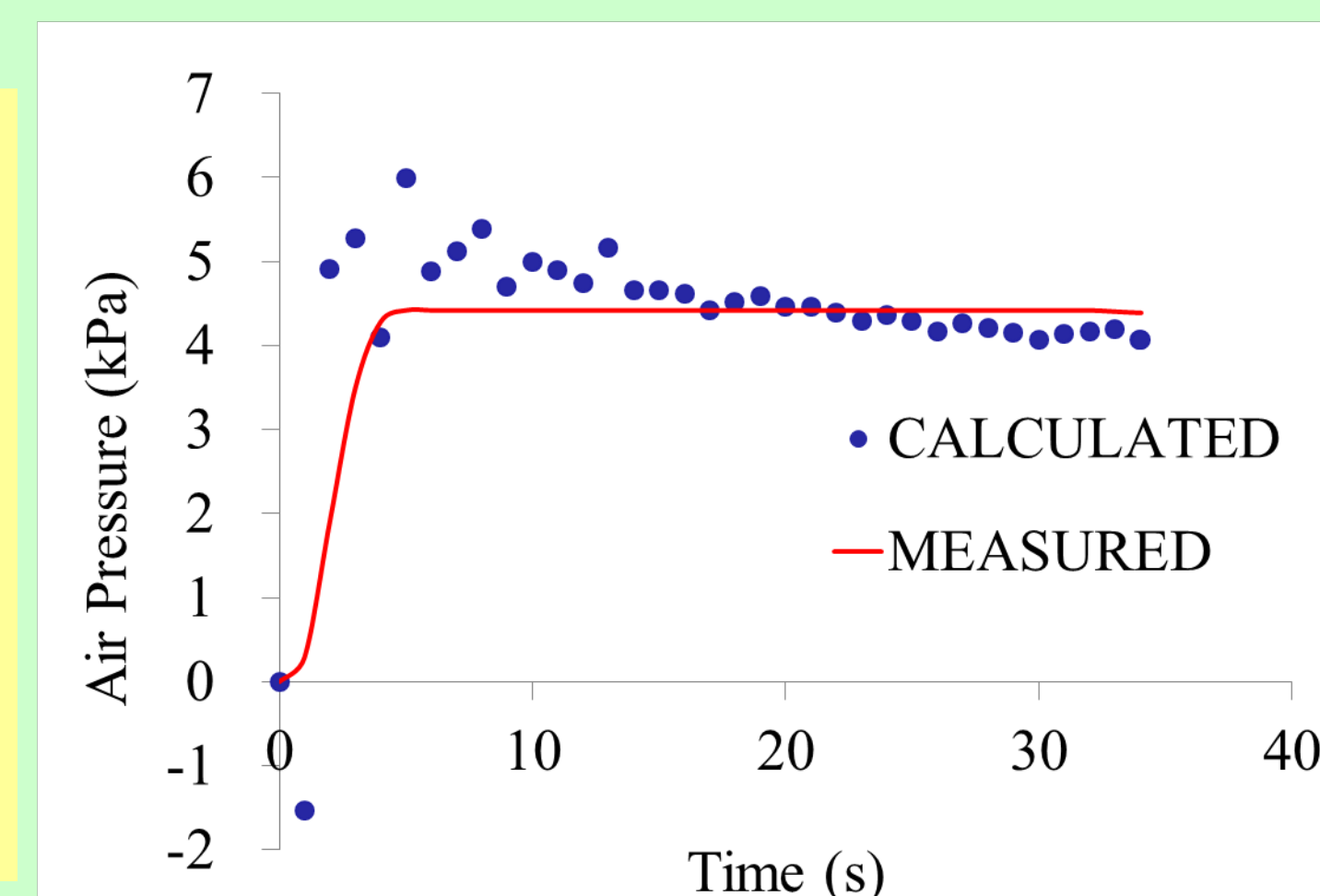
<Calculated air pressure ↔ Measured air pressure for 20kPa water infiltration rate>
