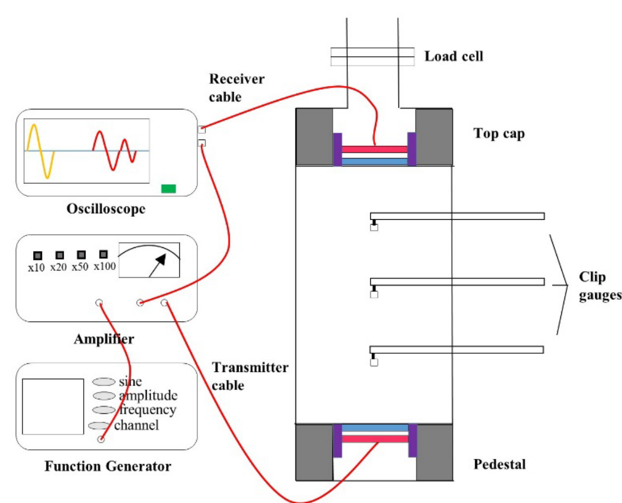
Layout of the apparatus
